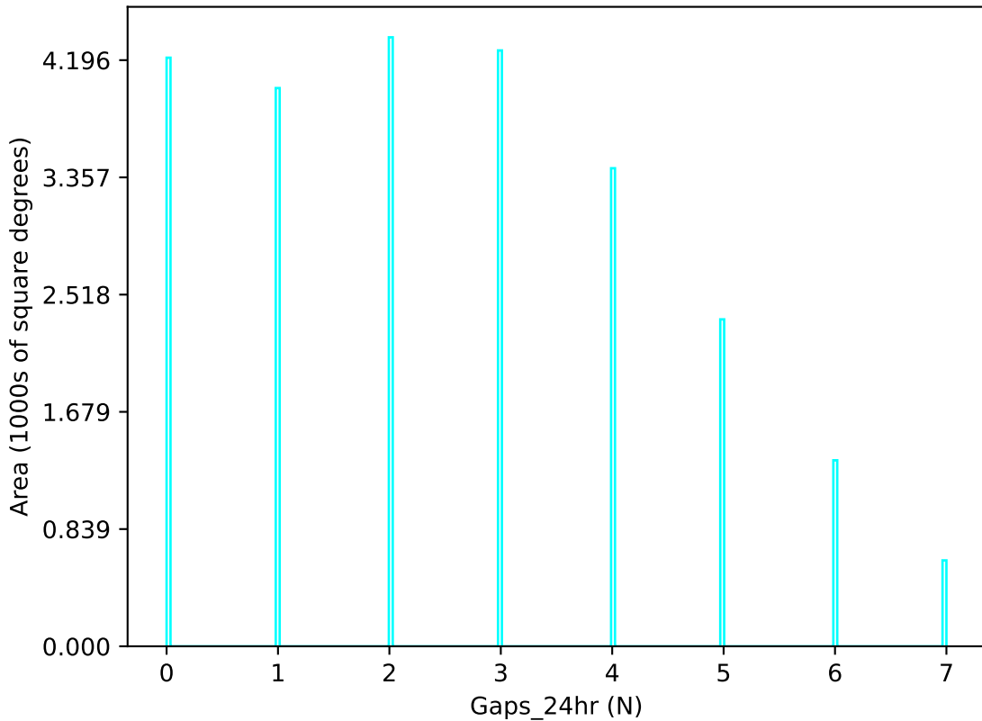
ddf_acor_sf15_lsf20_lsr50_v3.4_10yrs u band: Gaps_24hr
