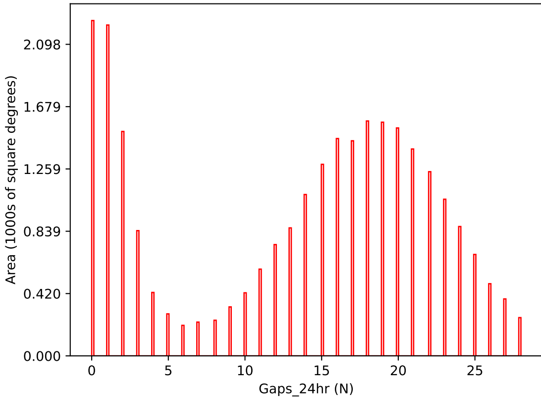
ddf_acor_sf15_lsf20_lsr50_v3.4_10yrs i band: Gaps_24hr
