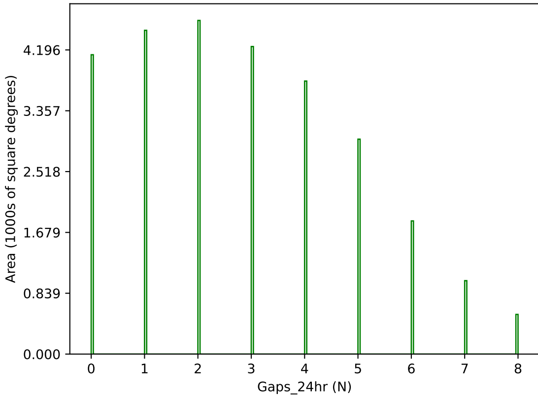
ddf_acor_sf15_lsf20_lsr50_v3.4_10yrs g band: Gaps_24hr
