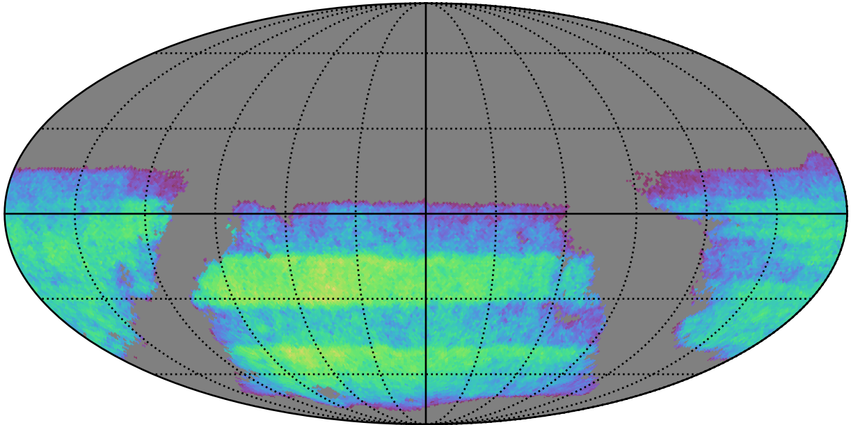
ddf_acor_sf15_lsf20_lsr50_v3.4_10yrs i band non-DD year 3: ExgalM5WithCuts
