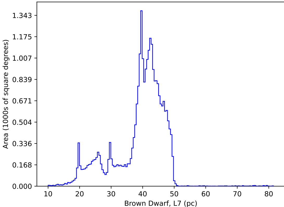
ddf_acor_sf15_lsf20_lsr50_v3.4_10yrs : Brown Dwarf, L7
