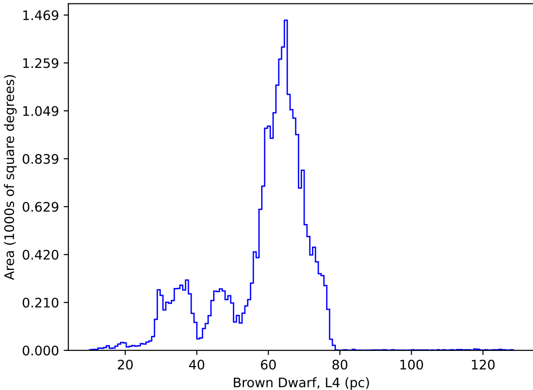
ddf_acor_sf15_lsf20_lsr50_v3.4_10yrs : Brown Dwarf, L4
