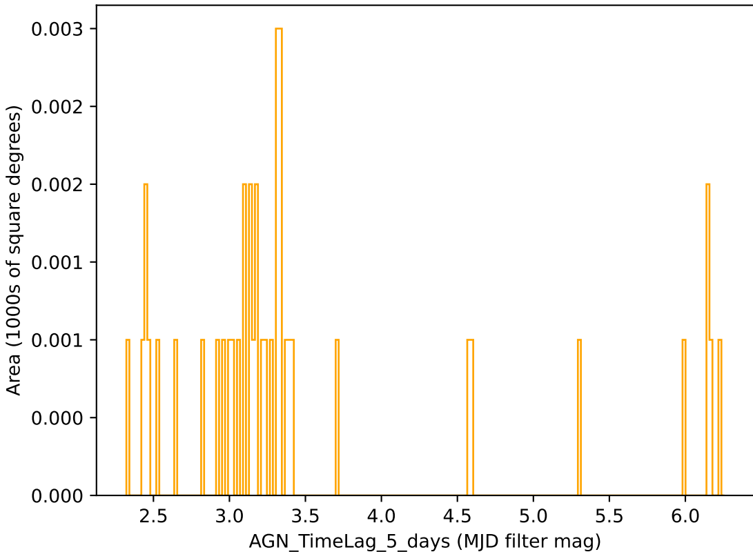
ddf_acor_sf15_lsf20_lsr50_v3.4_10yrs r band: AGN_TimeLag_5_days
