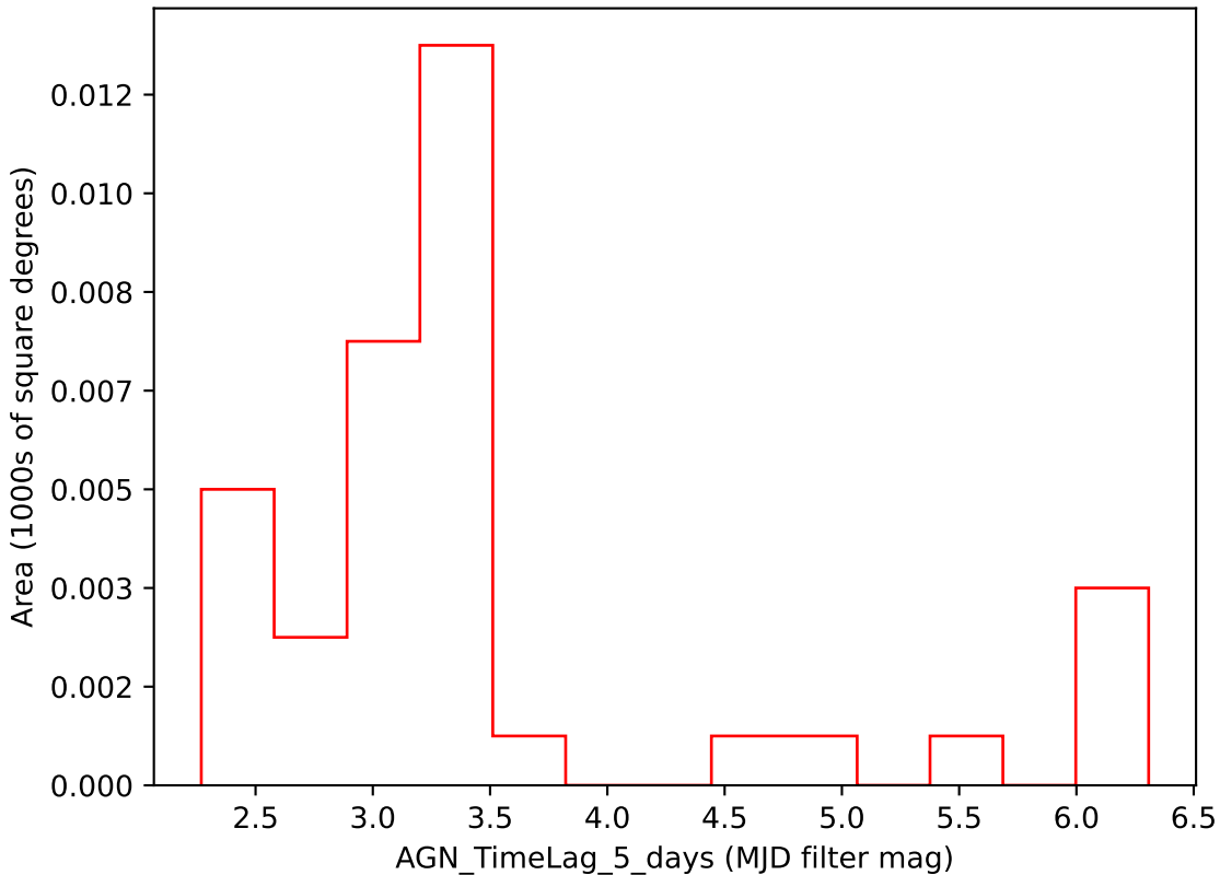
ddf_acor_sf15_lsf20_lsr50_v3.4_10yrs i band: AGN_TimeLag_5_days
