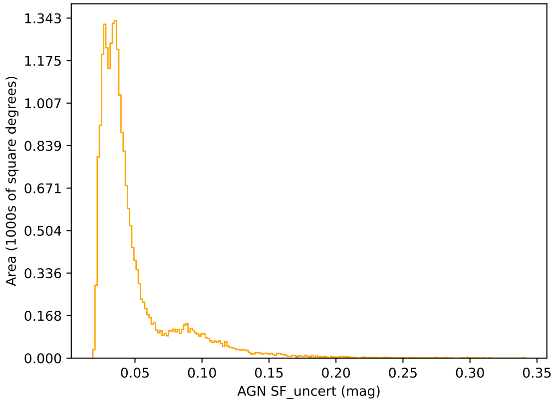
ddf_acor_sf15_lsf20_lsr50_v3.4_10yrs r band: AGN SF_uncert
