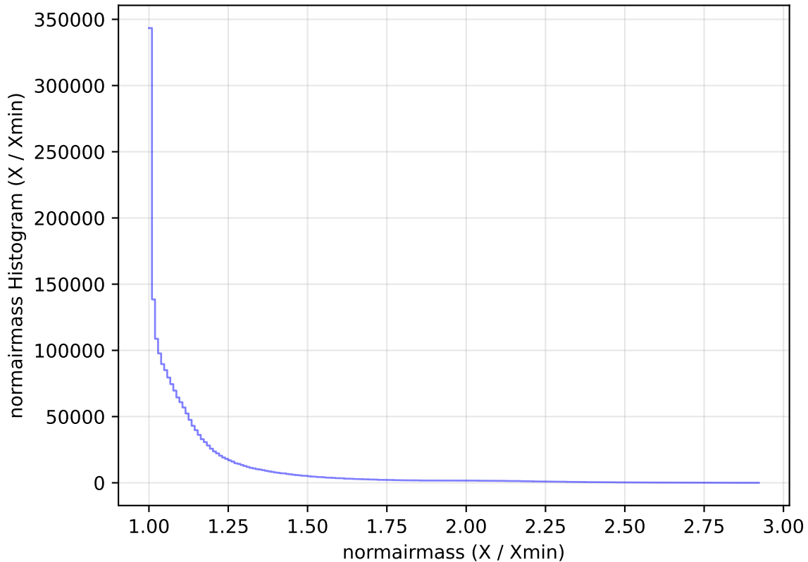
ddf_acor_sf15_lsf20_lsr50_v3.4_10yrs WFD all bands: normairmass Histogram
