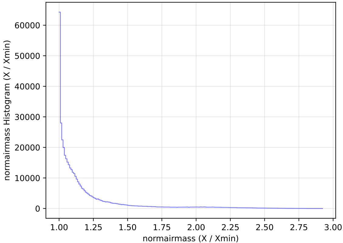
ddf_acor_sf15_lsf20_lsr50_v3.4_10yrs All sky z band: normairmass Histogram
