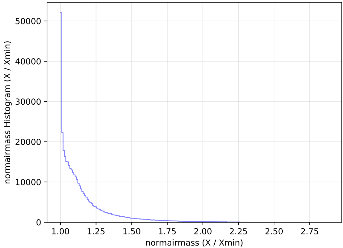
ddf_acor_sf15_lsf20_lsr50_v3.4_10yrs All sky y band: normairmass Histogram
