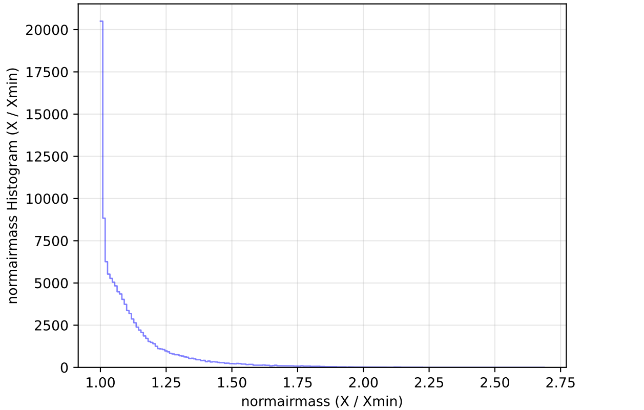
ddf_acor_sf15_lsf20_lsr50_v3.4_10yrs All sky u band: normairmass Histogram
