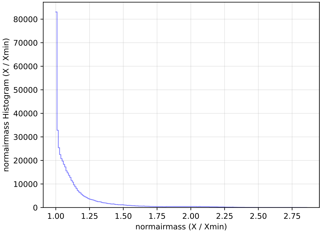
ddf_acor_sf15_lsf20_lsr50_v3.4_10yrs All sky r band: normairmass Histogram
