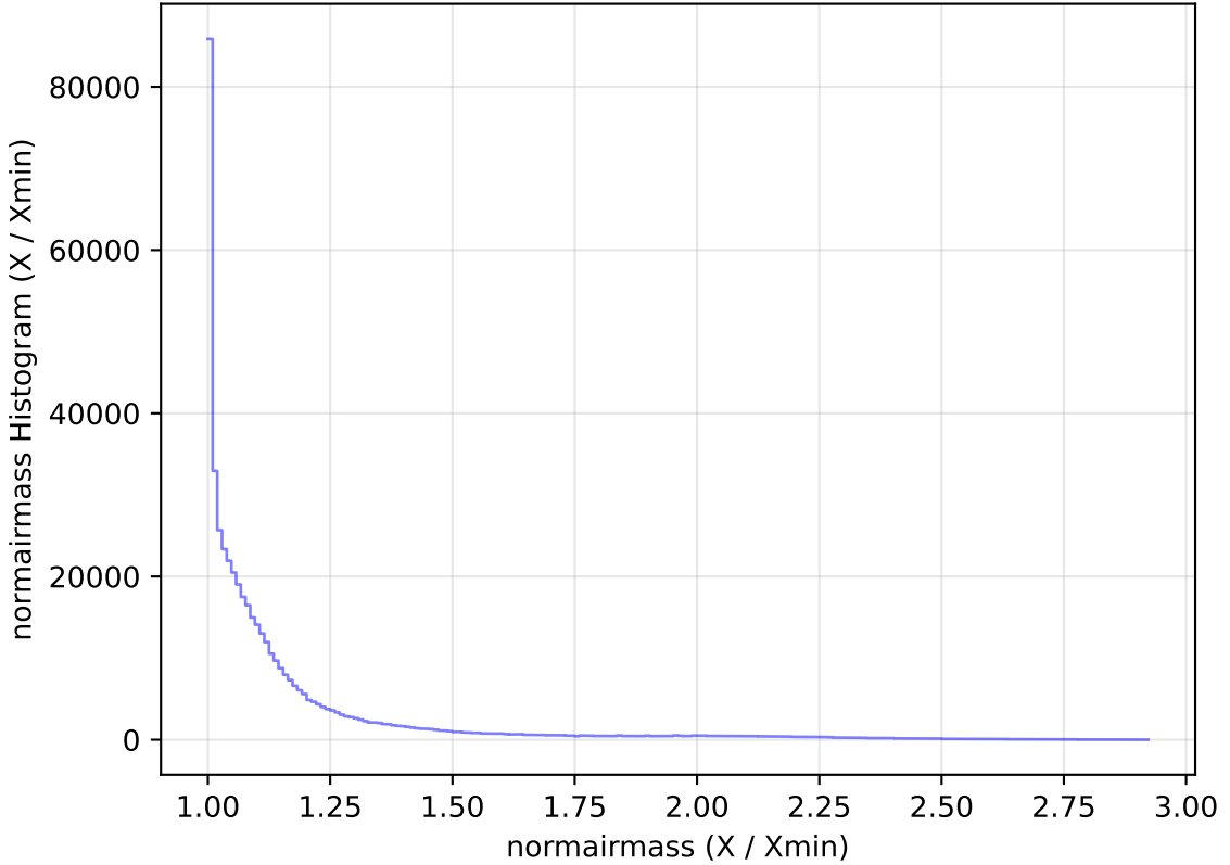
ddf_acor_sf15_lsf20_lsr50_v3.4_10yrs All sky i band: normairmass Histogram
