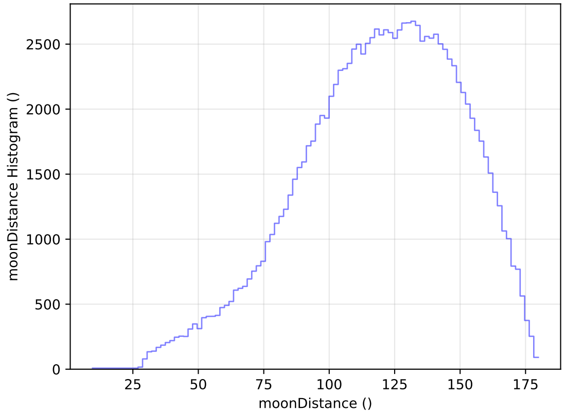
ddf_acor_sf15_lsf20_lsr50_v3.4_10yrs WFD u band: moonDistance Histogram
