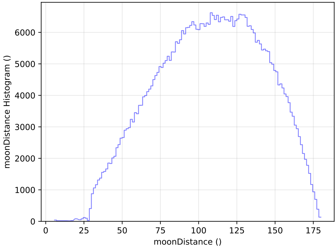
ddf_acor_sf15_lsf20_lsr50_v3.4_10yrs WFD r band: moonDistance Histogram
