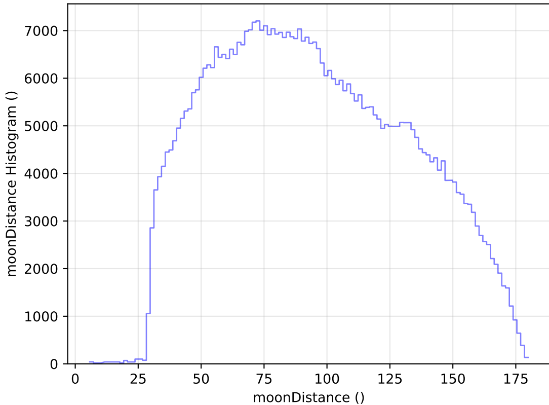
ddf_acor_sf15_lsf20_lsr50_v3.4_10yrs WFD i band: moonDistance Histogram
