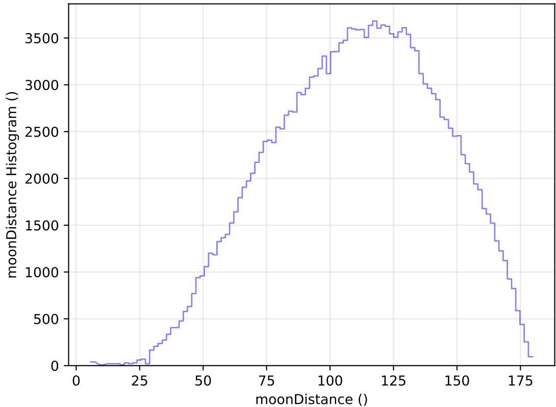
ddf_acor_sf15_lsf20_lsr50_v3.4_10yrs WFD g band: moonDistance Histogram
