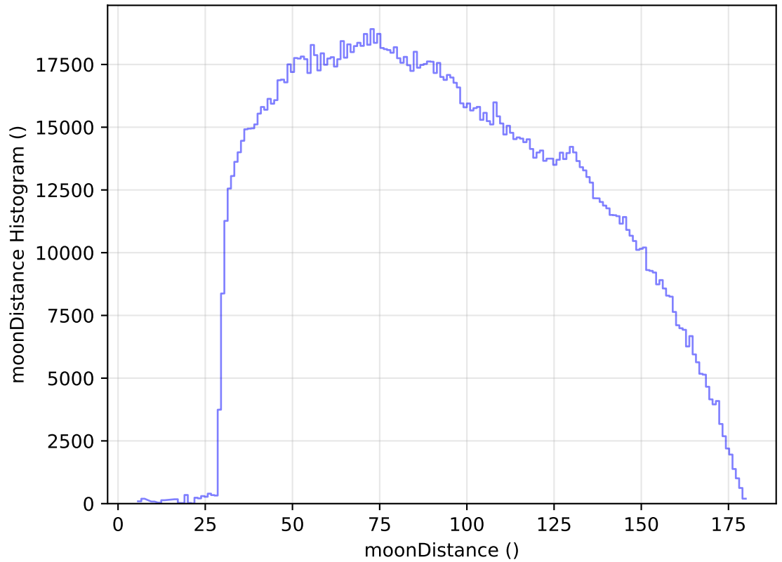
ddf_acor_sf15_lsf20_lsr50_v3.4_10yrs WFD all bands: moonDistance Histogram
