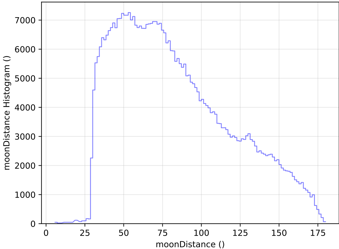
ddf_acor_sf15_lsf20_lsr50_v3.4_10yrs All sky z band: moonDistance Histogram
