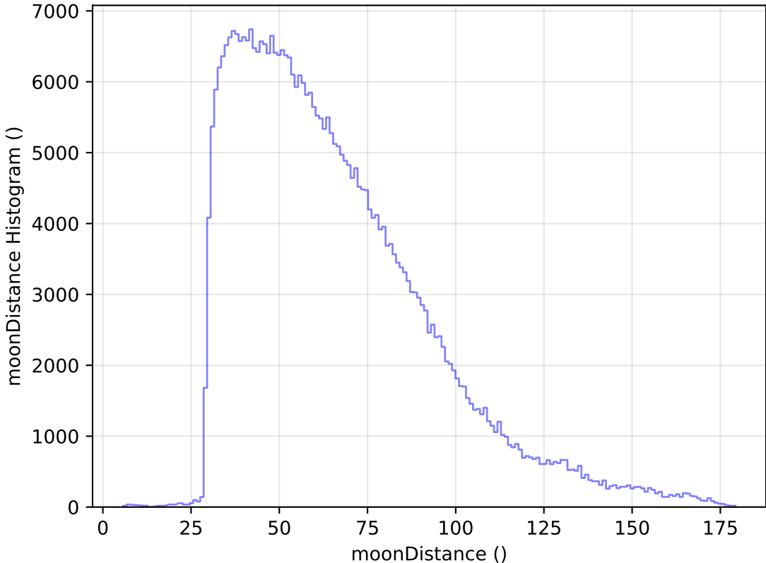
ddf_acor_sf15_lsf20_lsr50_v3.4_10yrs All sky y band: moonDistance Histogram
