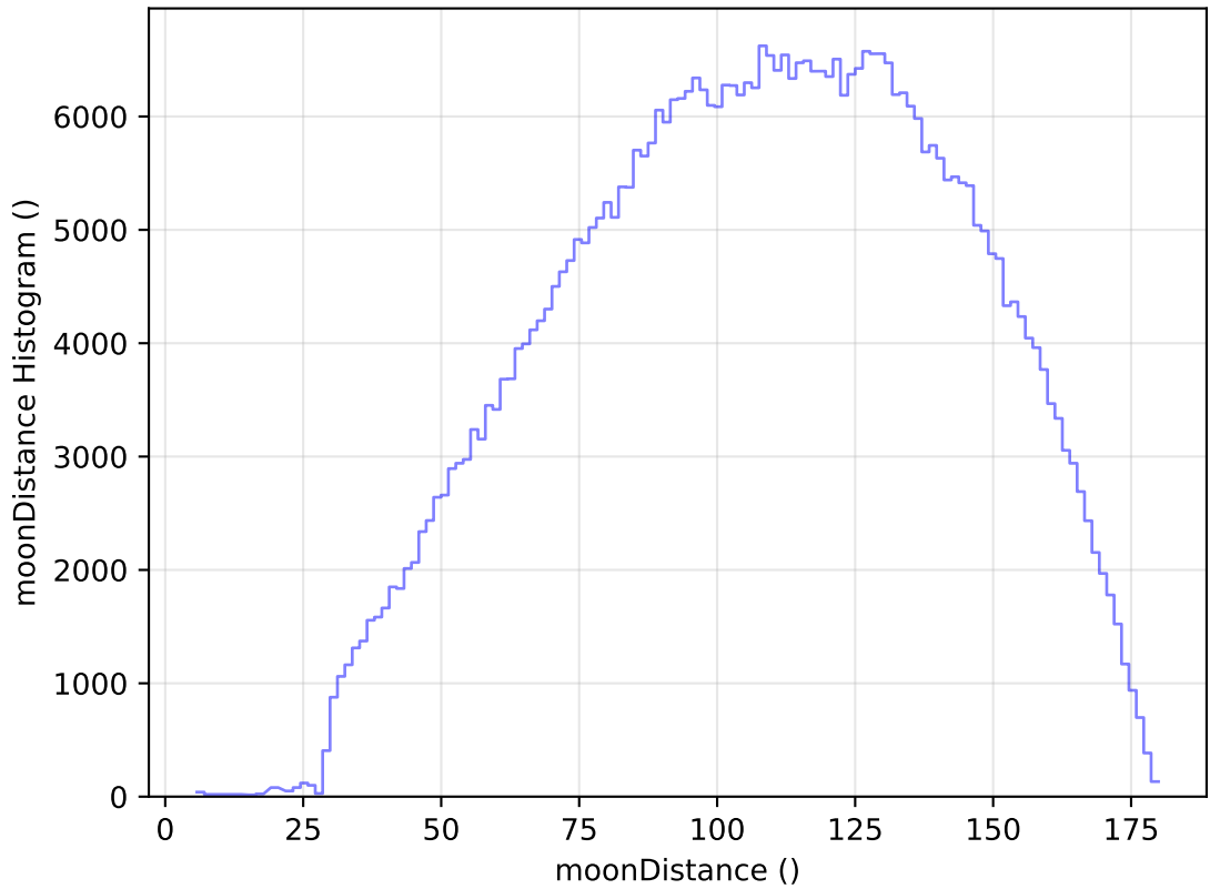
ddf_acor_sf15_lsf20_lsr50_v3.4_10yrs All sky r band: moonDistance Histogram
