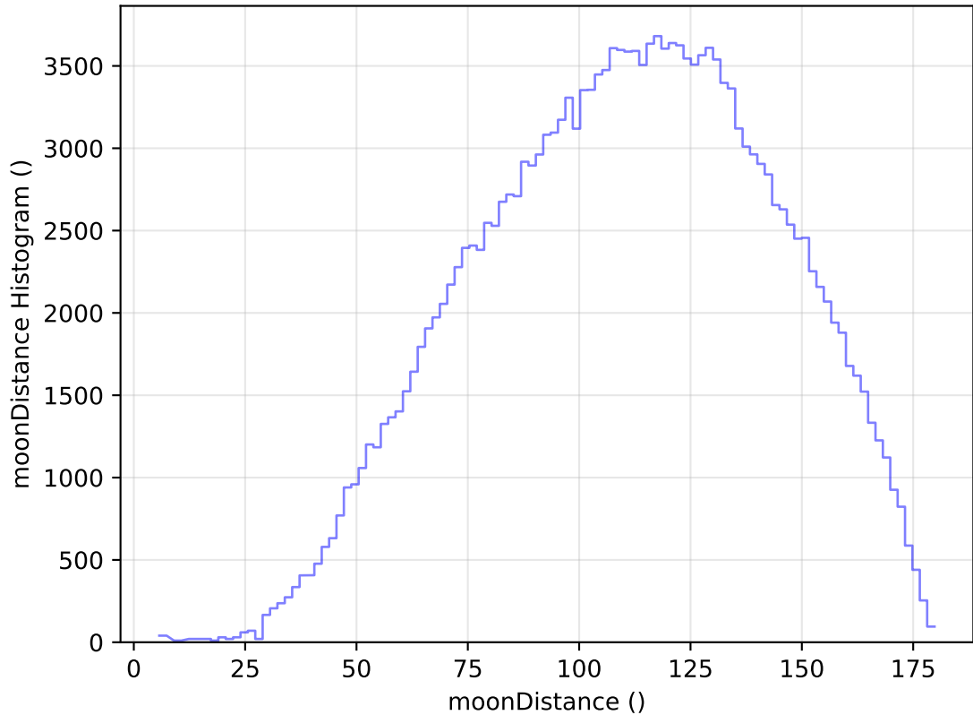
ddf_acor_sf15_lsf20_lsr50_v3.4_10yrs All sky g band: moonDistance Histogram
