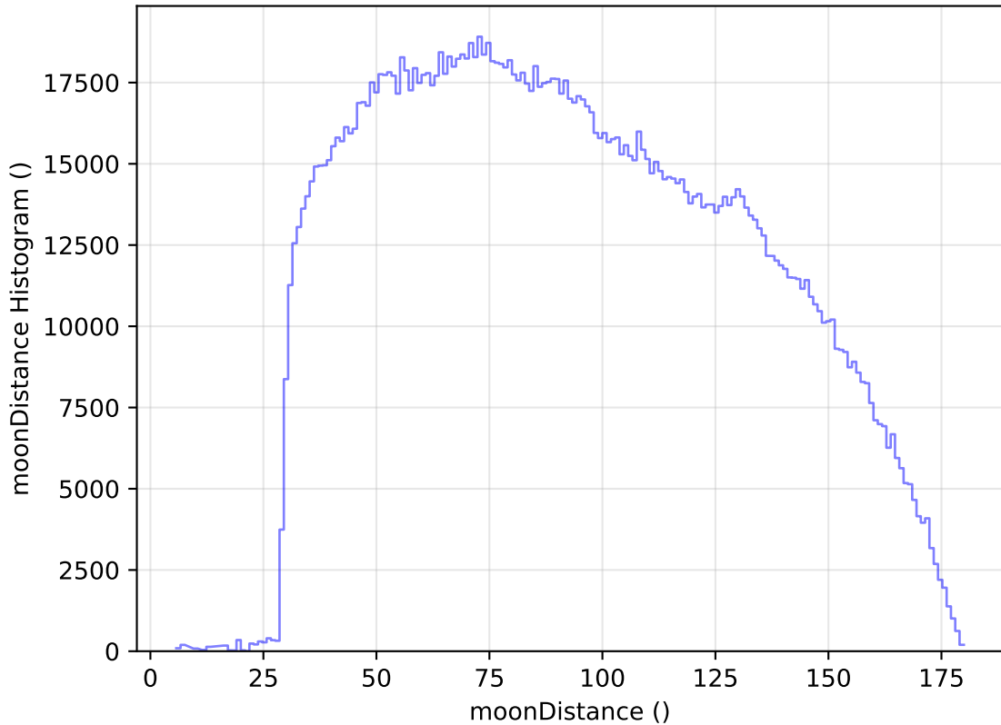
ddf_acor_sf15_lsf20_lsr50_v3.4_10yrs All sky all bands: moonDistance Histogram
