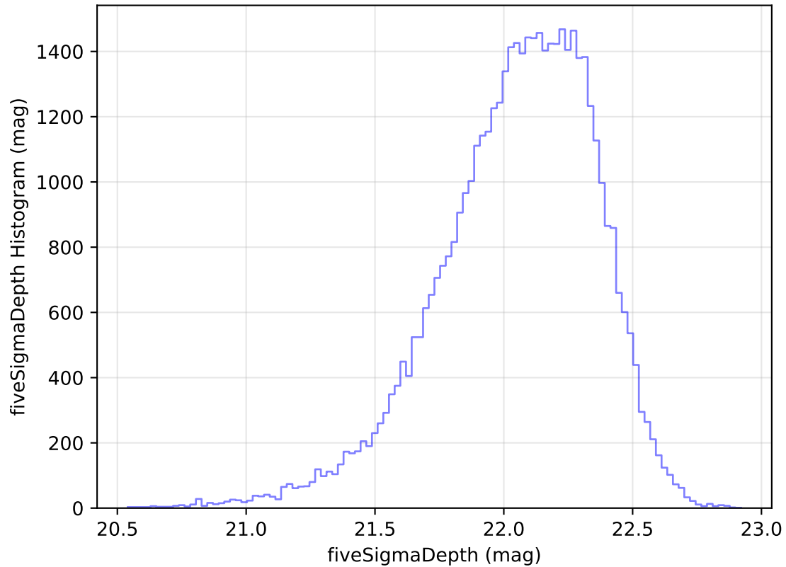
ddf_acor_sf15_lsf20_lsr50_v3.4_10yrs Yr 1 y band: fiveSigmaDepth Histogram
