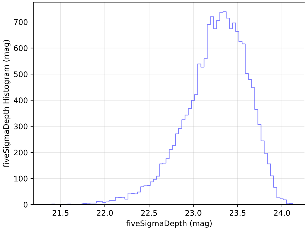
ddf_acor_sf15_lsf20_lsr50_v3.4_10yrs Yr 1 u band: fiveSigmaDepth Histogram
