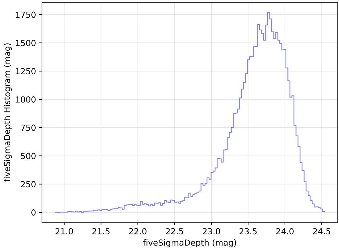
ddf_acor_sf15_lsf20_lsr50_v3.4_10yrs Yr 1 i band: fiveSigmaDepth Histogram
