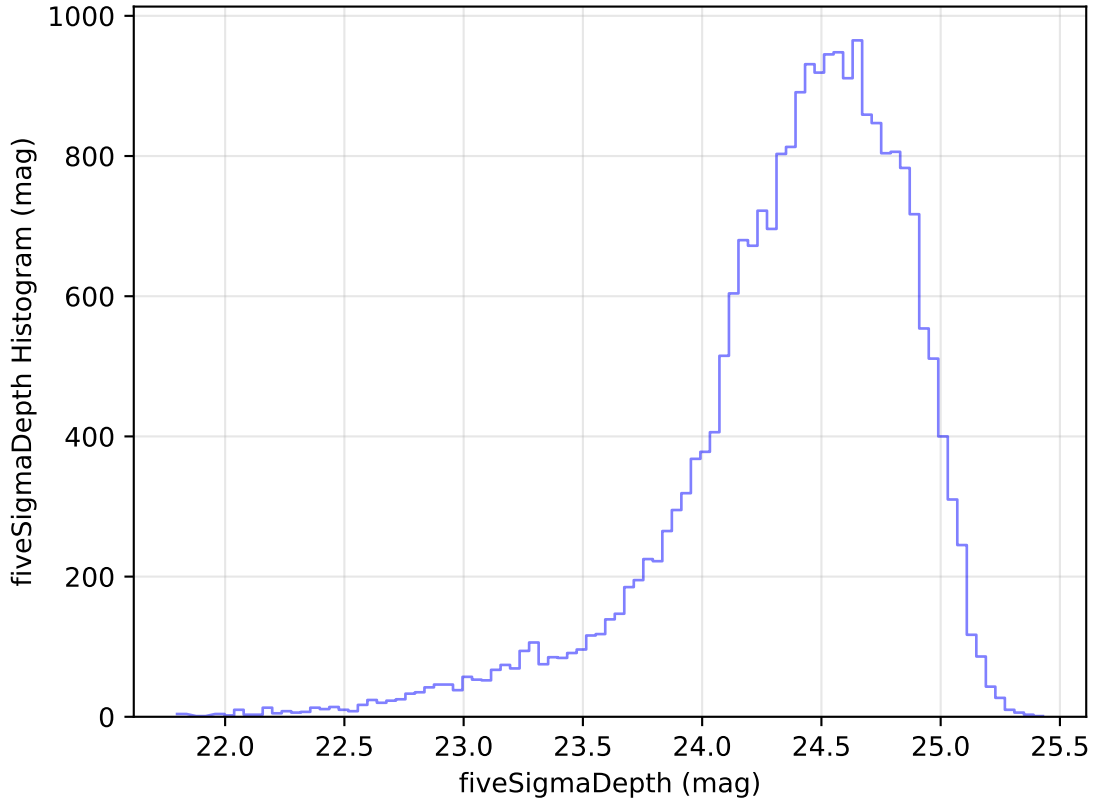
ddf_acor_sf15_lsf20_lsr50_v3.4_10yrs Yr 1 g band: fiveSigmaDepth Histogram
