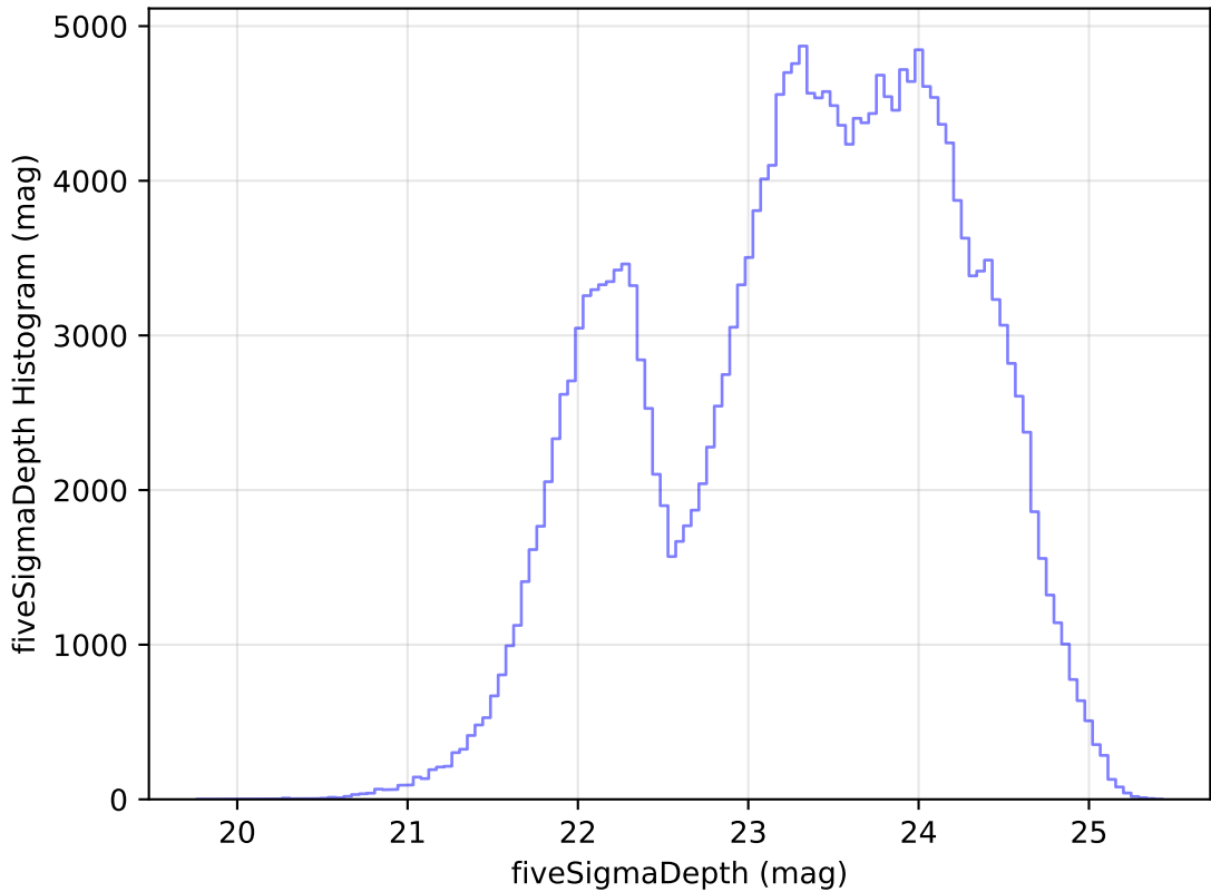
ddf_acor_sf15_lsf20_lsr50_v3.4_10yrs Yr 1 all bands: fiveSigmaDepth Histogram
