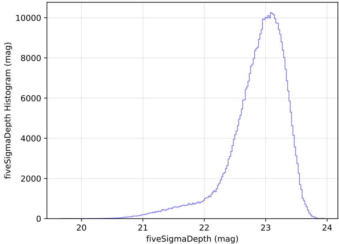
ddf_acor_sf15_lsf20_lsr50_v3.4_10yrs WFD z band: fiveSigmaDepth Histogram
