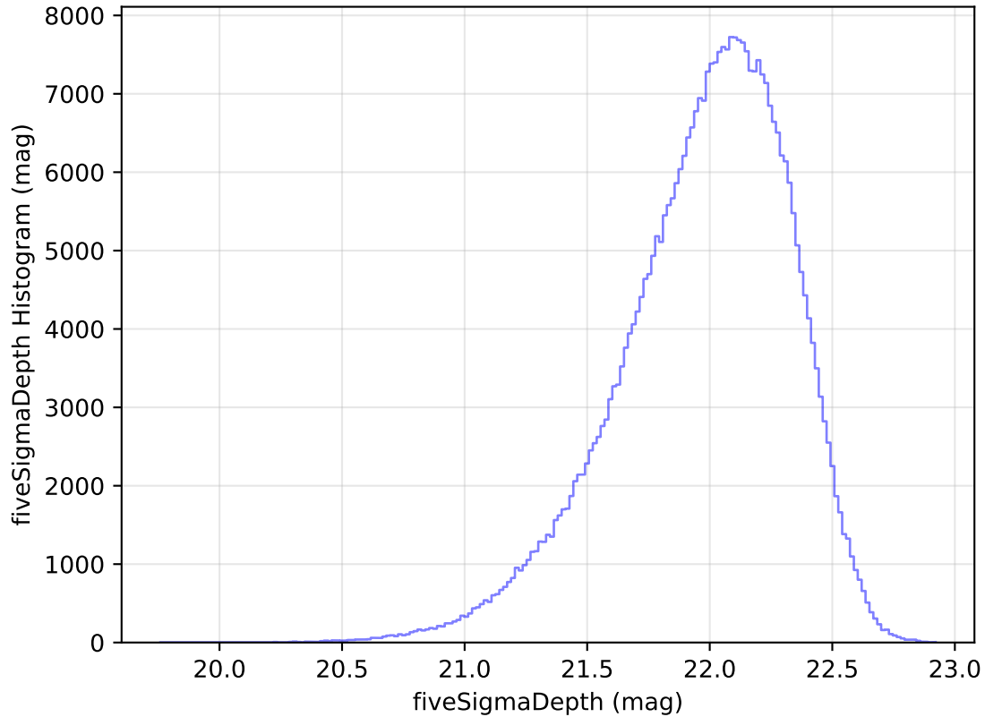
ddf_acor_sf15_lsf20_lsr50_v3.4_10yrs WFD y band: fiveSigmaDepth Histogram
