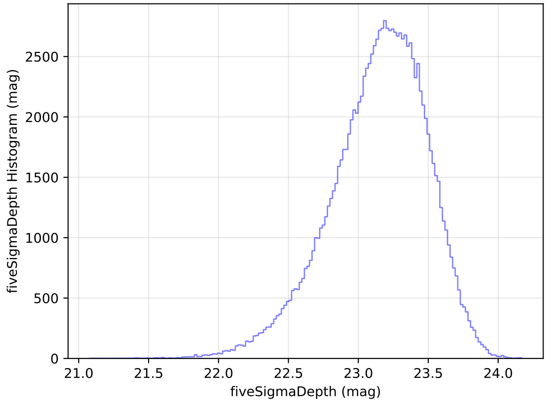
ddf_acor_sf15_lsf20_lsr50_v3.4_10yrs WFD u band: fiveSigmaDepth Histogram
