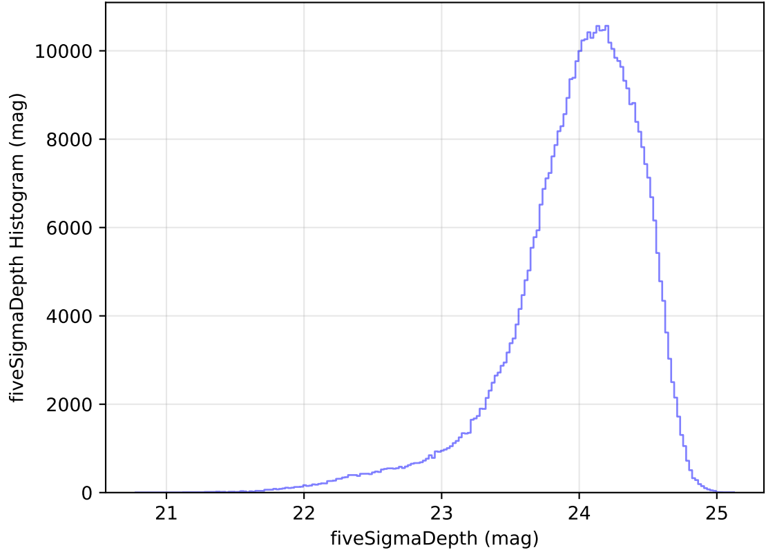
ddf_acor_sf15_lsf20_lsr50_v3.4_10yrs WFD r band: fiveSigmaDepth Histogram
