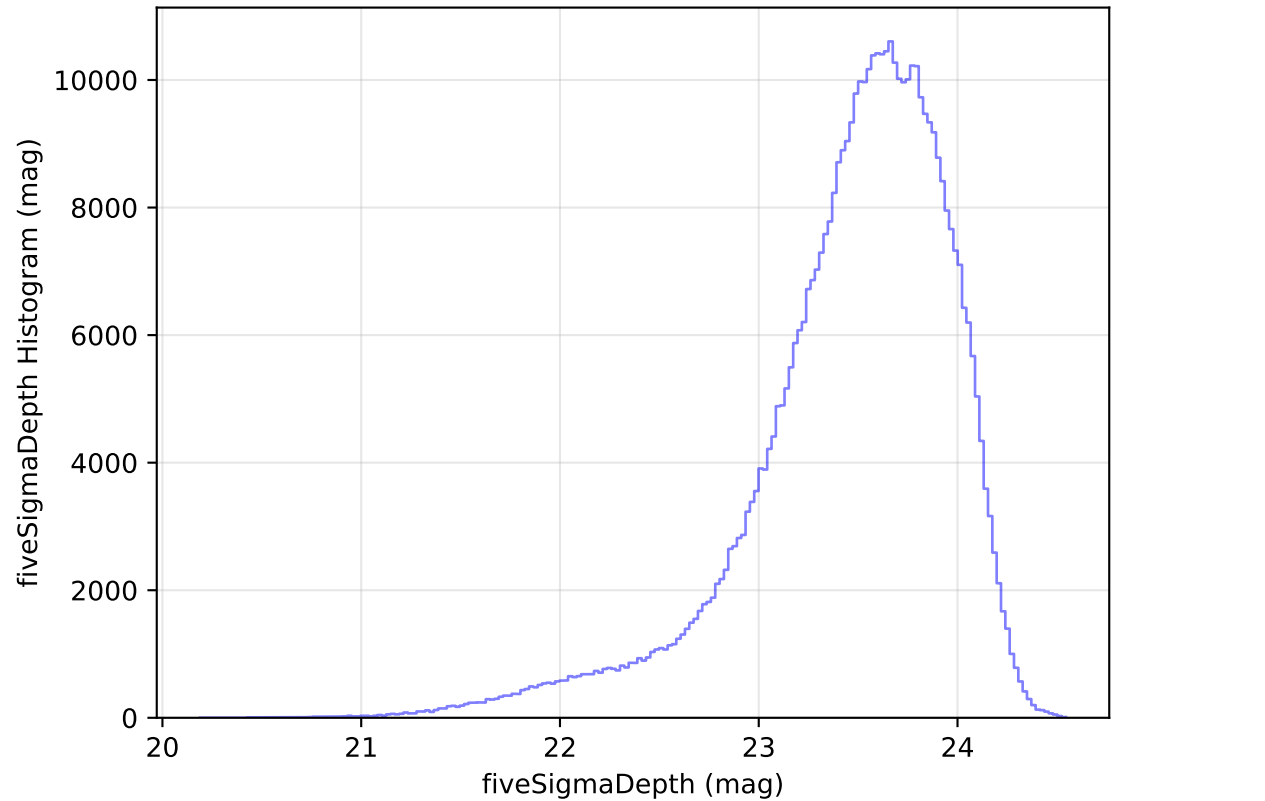
ddf_acor_sf15_lsf20_lsr50_v3.4_10yrs WFD i band: fiveSigmaDepth Histogram
