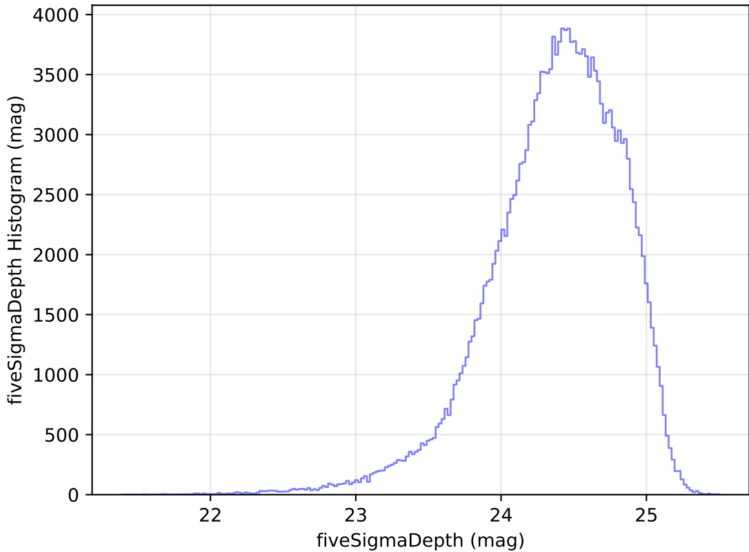
ddf_acor_sf15_lsf20_lsr50_v3.4_10yrs WFD g band: fiveSigmaDepth Histogram
