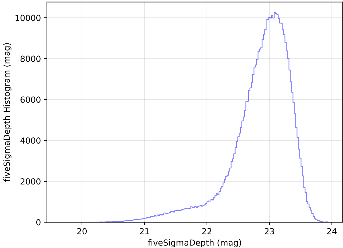
ddf_acor_sf15_lsf20_lsr50_v3.4_10yrs All sky z band: fiveSigmaDepth Histogram
