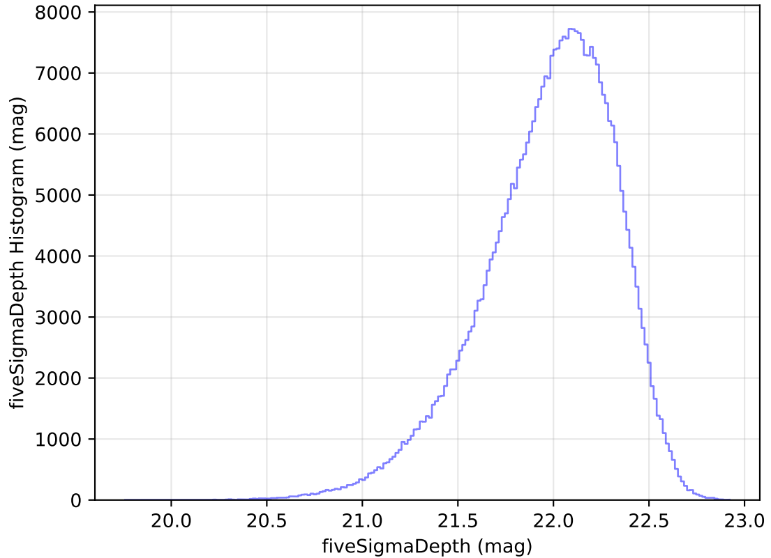
ddf_acor_sf15_lsf20_lsr50_v3.4_10yrs All sky y band: fiveSigmaDepth Histogram
