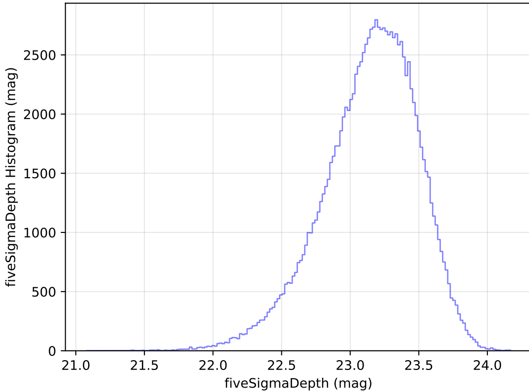
ddf_acor_sf15_lsf20_lsr50_v3.4_10yrs All sky u band: fiveSigmaDepth Histogram
