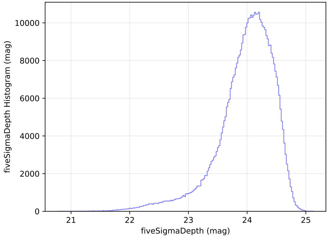
ddf_acor_sf15_lsf20_lsr50_v3.4_10yrs All sky r band: fiveSigmaDepth Histogram
