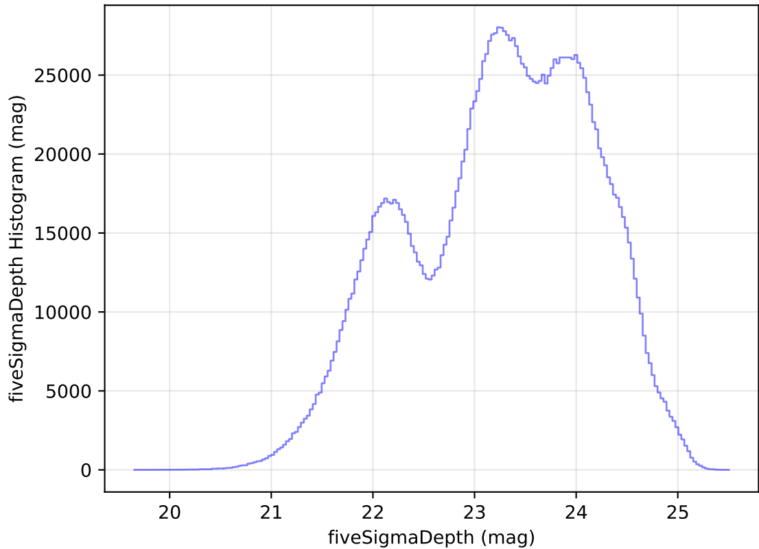
ddf_acor_sf15_lsf20_lsr50_v3.4_10yrs All sky all bands: fiveSigmaDepth Histogram
