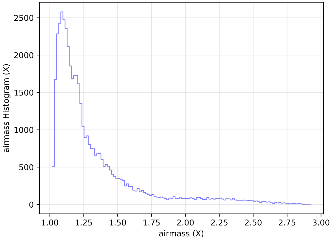
ddf_acor_sf15_lsf20_lsr50_v3.4_10yrs Yr 1 z band: airmass Histogram
