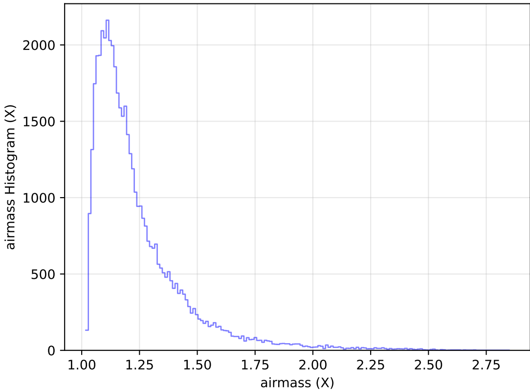
ddf_acor_sf15_lsf20_lsr50_v3.4_10yrs Yr 1 y band: airmass Histogram
