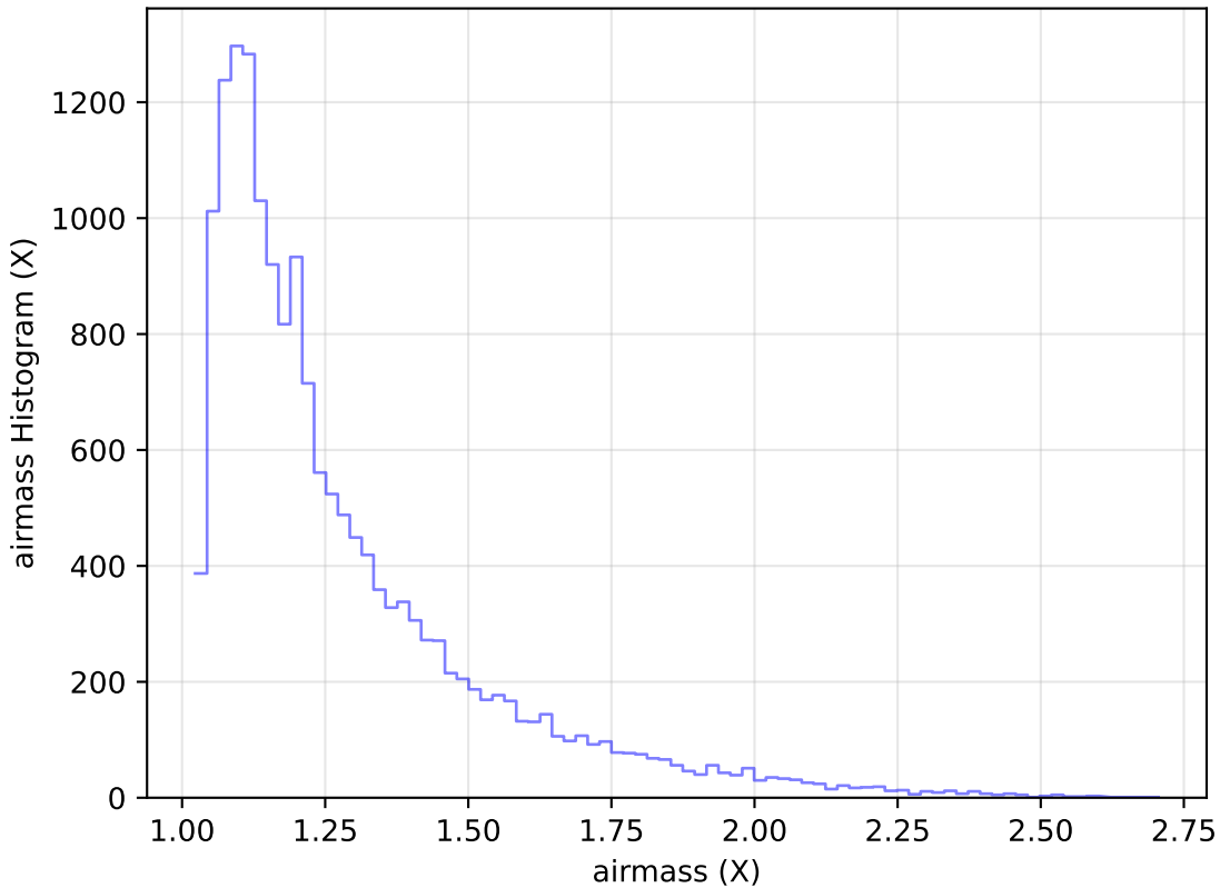
ddf_acor_sf15_lsf20_lsr50_v3.4_10yrs Yr 1 u band: airmass Histogram
