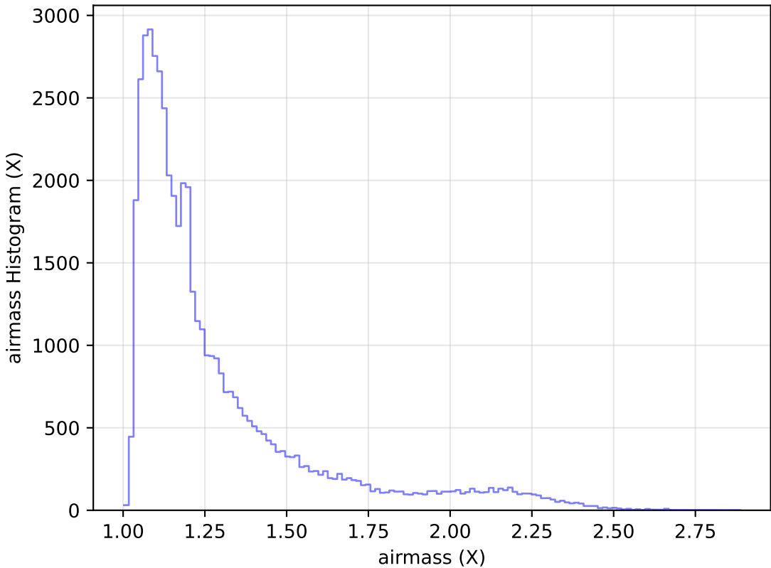
ddf_acor_sf15_Isf20_Isr50_v3.4_10yrs Yr 1 r band: airmass Histogram
