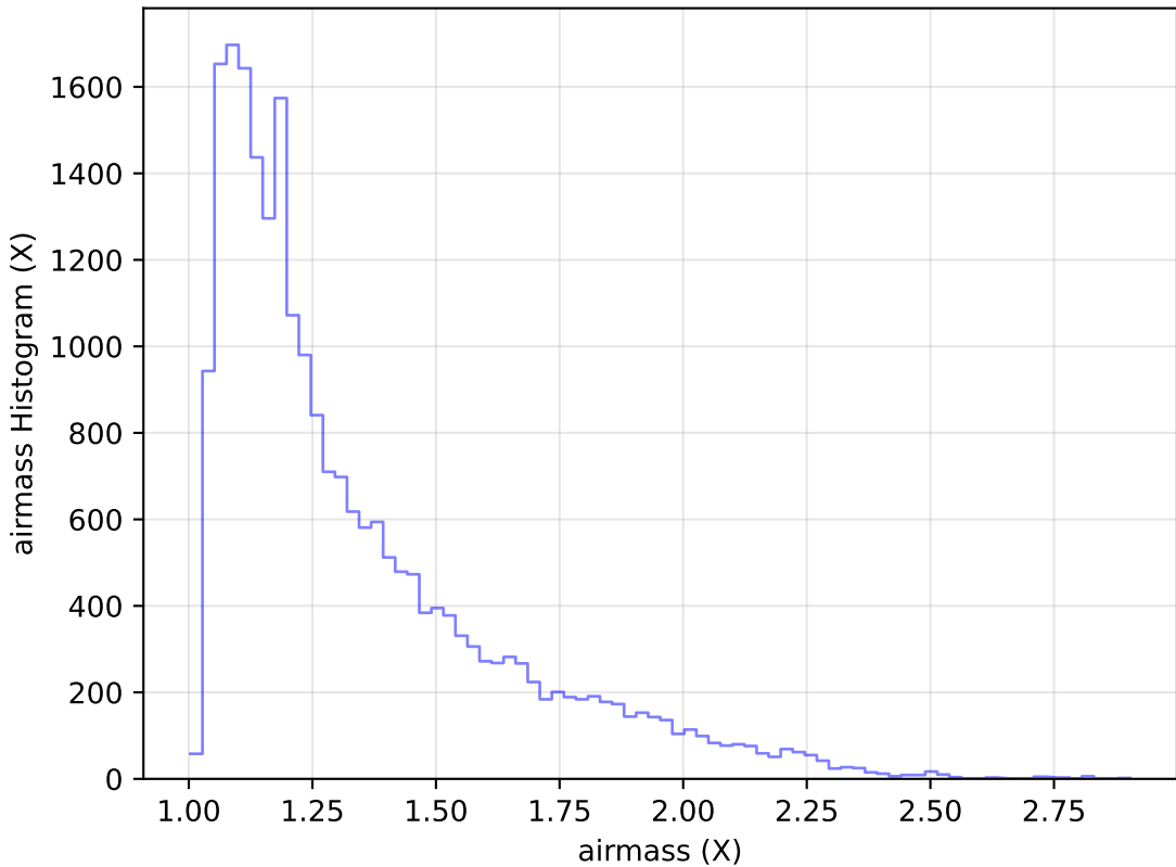
ddf_acor_sf15_lsf20_lsr50_v3.4_10yrs Yr 1 g band: airmass Histogram
