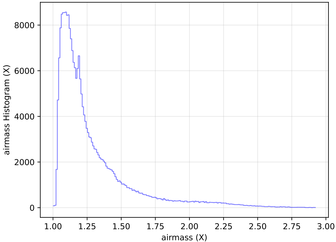
ddf_acor_sf15_lsf20_lsr50_v3.4_10yrs Yr 1 all bands: airmass Histogram
