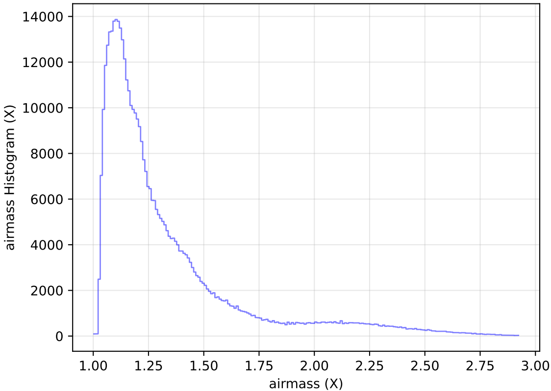
ddf_acor_sf15_lsf20_lsr50_v3.4_10yrs WFD z band: airmass Histogram
