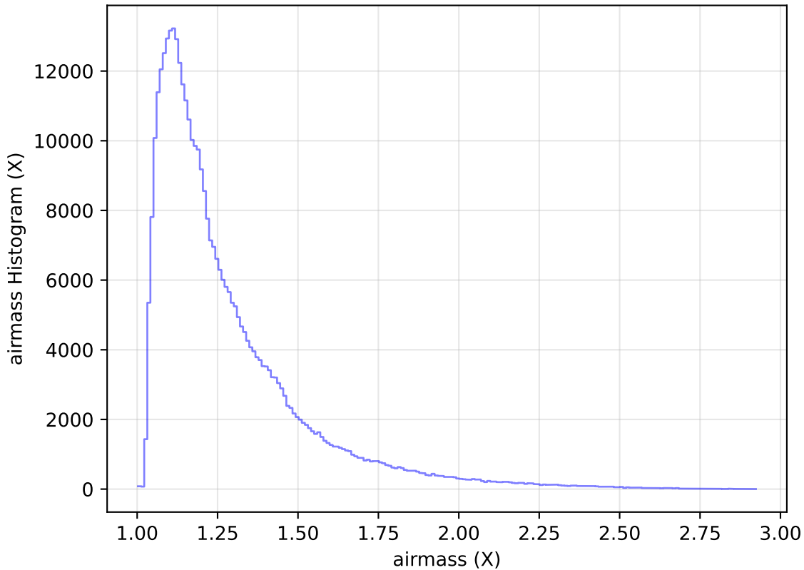
ddf_acor_sf15_lsf20_lsr50_v3.4_10yrs WFD y band: airmass Histogram
