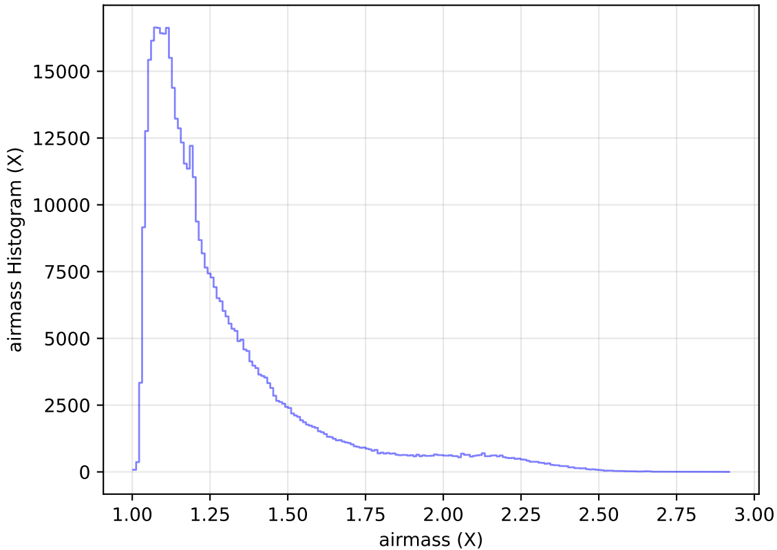
ddf_acor_sf15_lsf20_lsr50_v3.4_10yrs WFD r band: airmass Histogram
